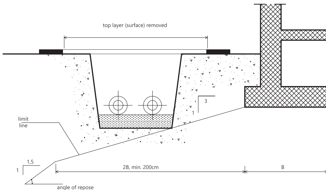
Figure 04 (reference drawing)
